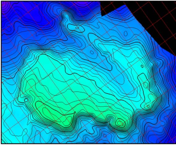
Figure 3 – Beehive on reprocessed 2D seismic
