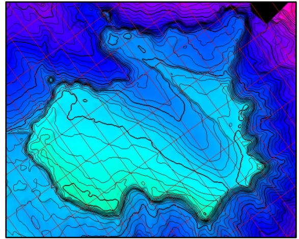
Figure 4 – Beehive on 3D seismic
